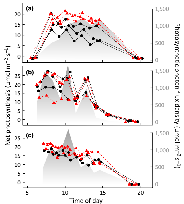
FIGURE 4 Diurnal patterns in net photosynthesis of Ochroma pyramidale saplings grown at ambient (black circles, solid black lines) and elevated (red triangles, dashed red lines) night temperatures in three experiments (a–c). Values are means of measurements on three leaves per plant. Grey areas indicate photosynthetic photon flux density recorded at the time of photosynthesis measurements (secondary y axis)
